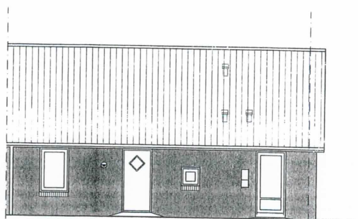
TYPE 82 FACADE MOD ADGANGSSIDE
